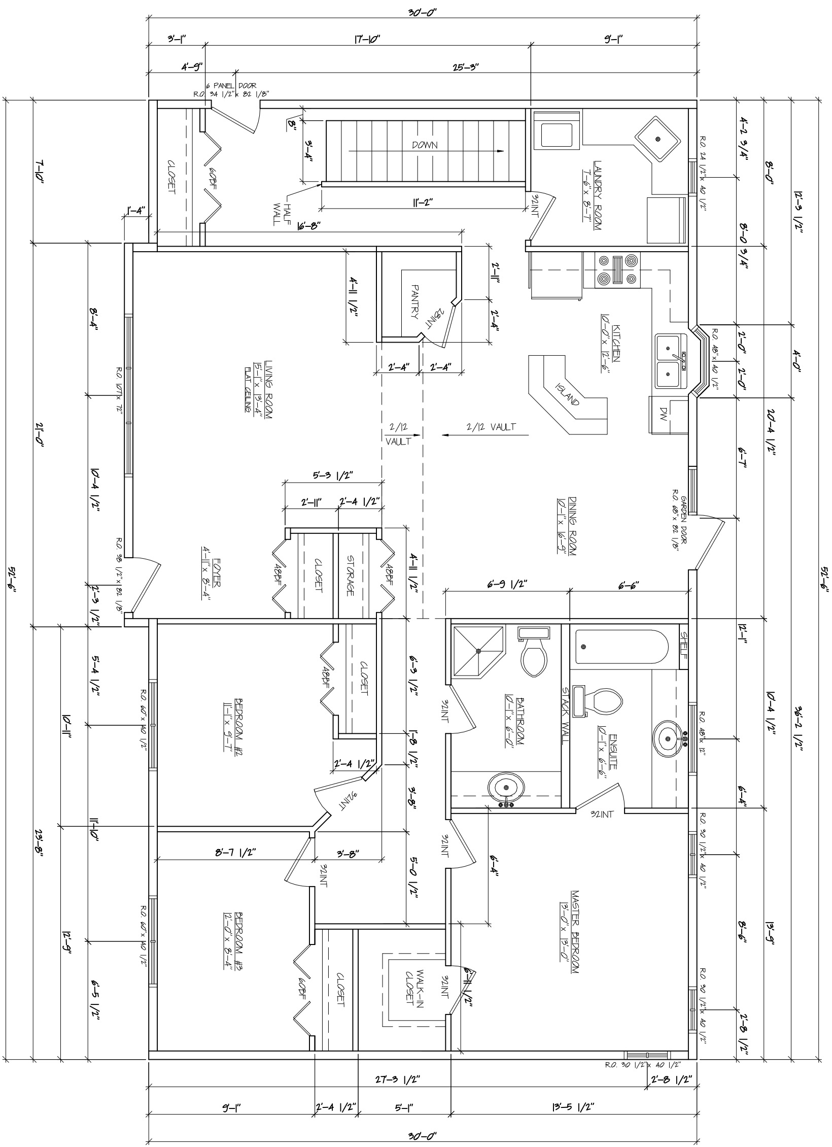
MAIN FLOOR PLAN SCALE: 3/16" = 1'-0"
